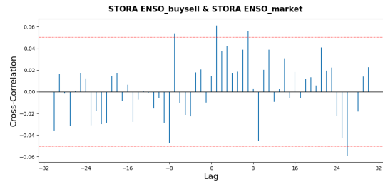
Figure 15: Cross-Correlation function for STORA ENSO.
