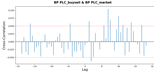
Figure 14: Cross-Correlation function for BP PLC.
