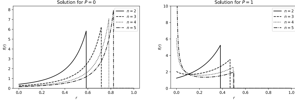
Figure 4: We observe a clear difference between the cases P = 0 (no penalty) and P = 1 (presence of a penalty). In both cases, the cutoff increases. However, the average risk seems to decrease sharply when there is a nonzero penalty with a mode at r = 0 .
