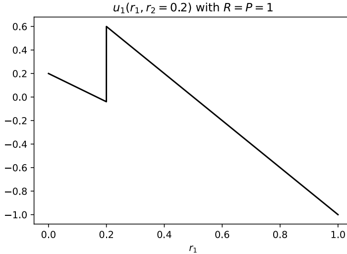
Figure 1: Reward function
