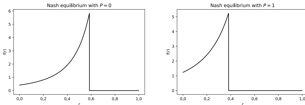
Figure 2: Nash equilibrium
