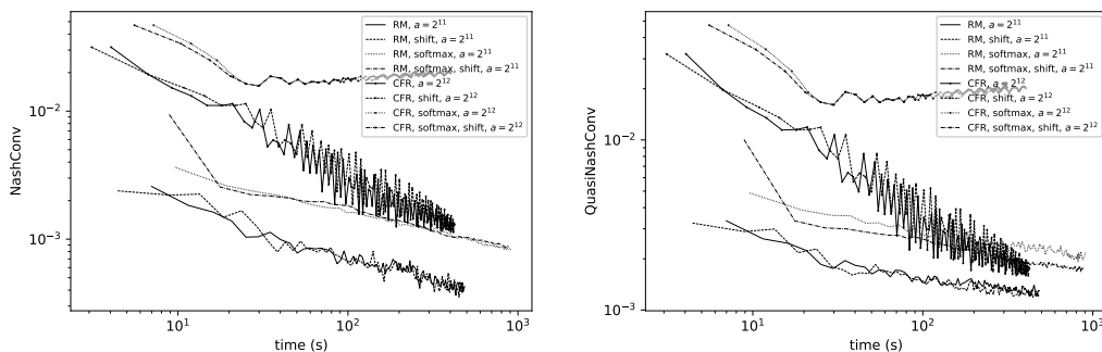
Figure 9: We evaluate the performance of different algorithms in finding the Nash equilibrium of the Cfr game in the standard setting with P = R = 1, \tau = 0 , and \rho = 0 , without sharing. We reduce the game to a grid of a = 2^{12} actions, and evaluate the QUASINASHCONV metric on 2^{15} points. The algorithms are run for 10^4 iterations, where an iteration is defined as an update to the strategy. For CFR, an iteration involves updating the regrets based on the counterfactual outcomes of the game, while for regret matching, an iteration is defined as a steps of the sampling, play, and update process. Both CFR and regret matching do \mathcal{O}(a^2) operations per iteration. We do not include the computation of the utility matrix in the computation time.
