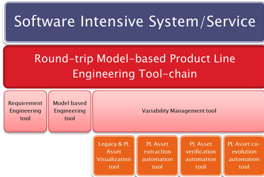
Figure 2: REVAMP approach
