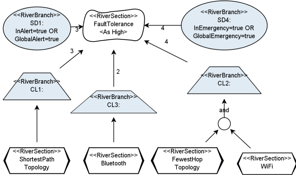
Figure 11: A subset of the SG satisficing view of running example
