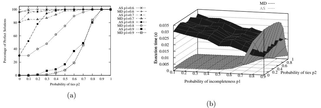
Fig. 3: AS vs. MD: a) quality of solutions b) execution time.
