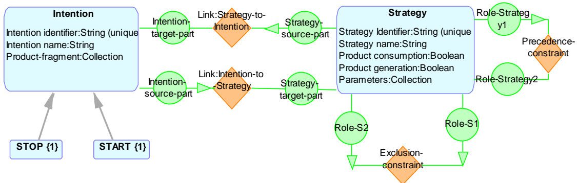
Figure 3. Map process meta-model defined in GOPRR
