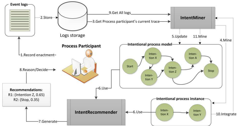
Fig. 1. FlexPAISSeer approach
