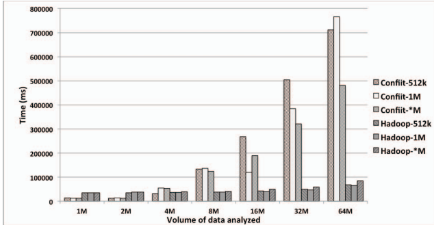
Figure 3. Comparison between Confiiit and Hadoop over 16 nodes
