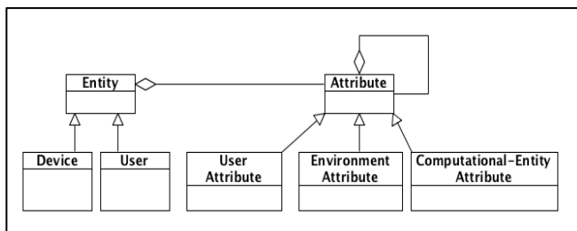
Figure 5. Context Model
