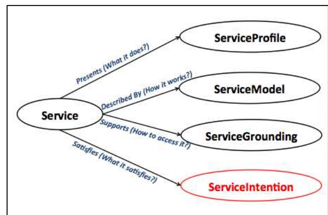
Figure 8. Service intention Description in OWL-S
