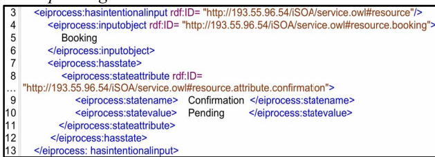
Figure 5: Intentional input in OWL-S process model
