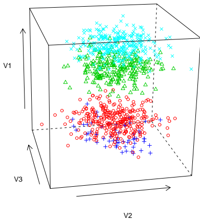
Figure 7: Projection of the data in the 3 first principal components of PCA (left) and in the discriminant subspace estimated by Fisher-EM with the \text{DLM}_{[\alpha_k \beta]} .
