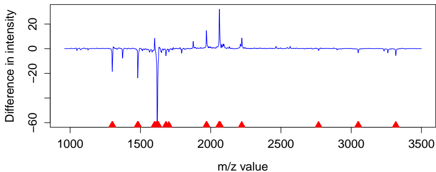
Figure 10: Difference between the mean spectra of the classes cancer and control (cancer - control) and most discriminative variables (indicated by red triangles).
