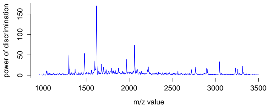
Figure 9: Discrimination power of the original variables: correlation between original variables and the discriminative subspace on an arbitrary scale.
